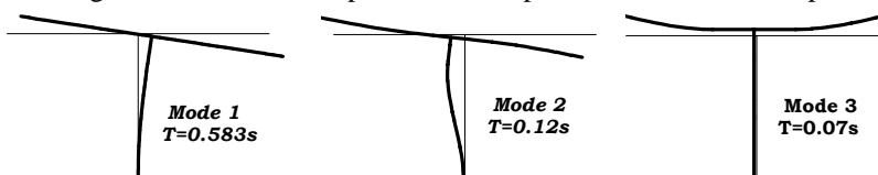
Figure 2 – Modal shapes
